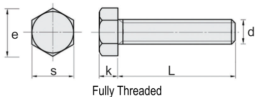
DIN 933 (Fully Threaded)
